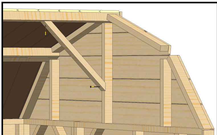
Front Gable
