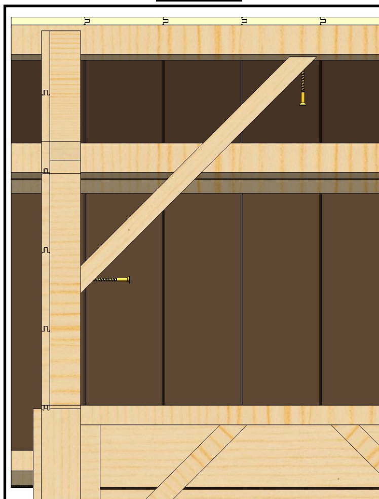
Rear Gable
